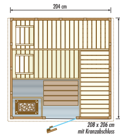
Blockbohle-W Gerade
